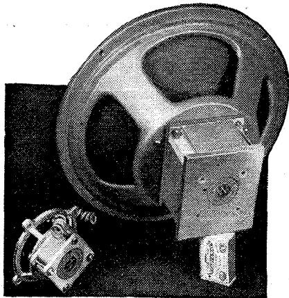
Wharfedale PA12 loudspeaker chassis and 3½ in. Midget microphone - LS unit.
