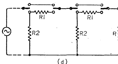
Fig. 6. Development of the "inverted L" attenuator. By means of the switches shown, any desired amount of attenuation can be obtained in steps. The dotted line indicates where other "L" cells may be added.
