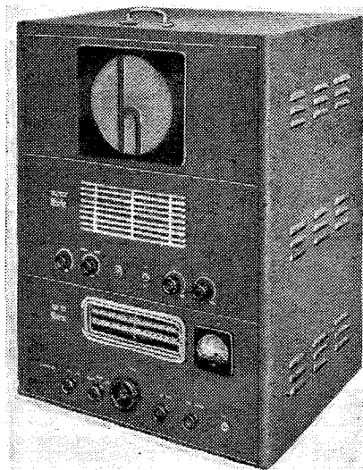
FM/AM RECEIVER. Hallicrafters' Model RSC-2 receiver, which is intended for hotel and hospital installations, comprises FM and AM tuners, a high-fidelity 25-watt amplifier, and monitoring speaker. Change-over from FM to AM is linked with the waveband switch. Provision is made for using a microphone and pick-up.
