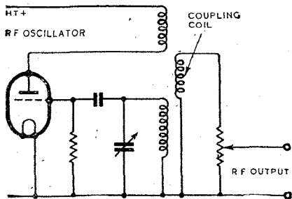
Fig. 5. This type of output control is used in several inexpensive test oscillators, and is satisfactory for rough general service work.
