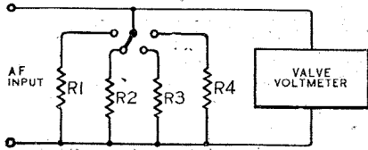
Fig. 1. A simple output meter. The resistances R1, R2, R3, R4 may be of ohmic values corresponding to the impedances of the various normal loads in the anode circuits of output stages, e.g., 2Ω and 8Ω to represent speech coils; 2,000Ω and 12,000Ω to represent primaries of speaker transformer. The valve voltmeter must be able to cover the ranges of voltage developed across these resistances.
