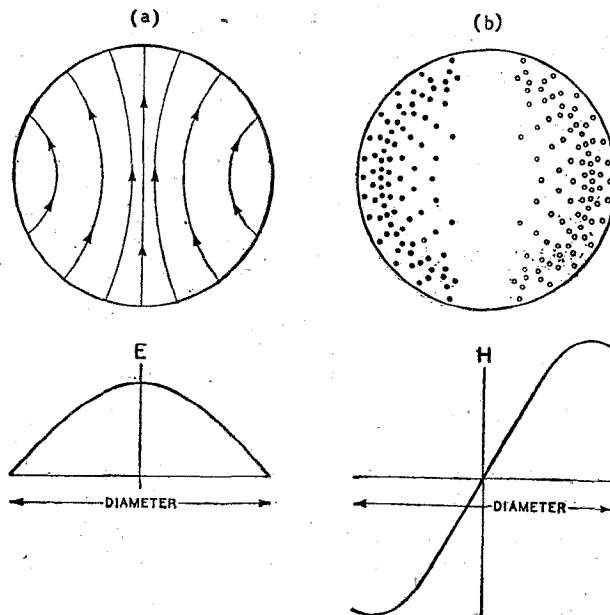
Fig. 4. (after Hansen). One mode of oscillation of a spherical resonator. (a) Shows the electric lines at the instant when the magnetic field is zero. (b) Shows the situation \frac{1}{4} cycle later, when the energy is in the magnetic field which is perpendicular to the plane of this sectional diagram. The intensity and distribution of each field are also shown graphically.
