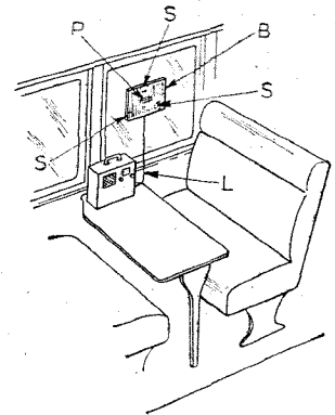
Mounting a detachable frame aerial.
