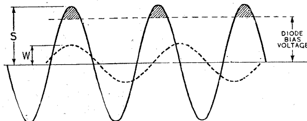
Fig. 1.—Diode rectification with a strong "wanted" signal and weaker interference of different frequency. The diode conducts during parts of cycle shown shaded.
